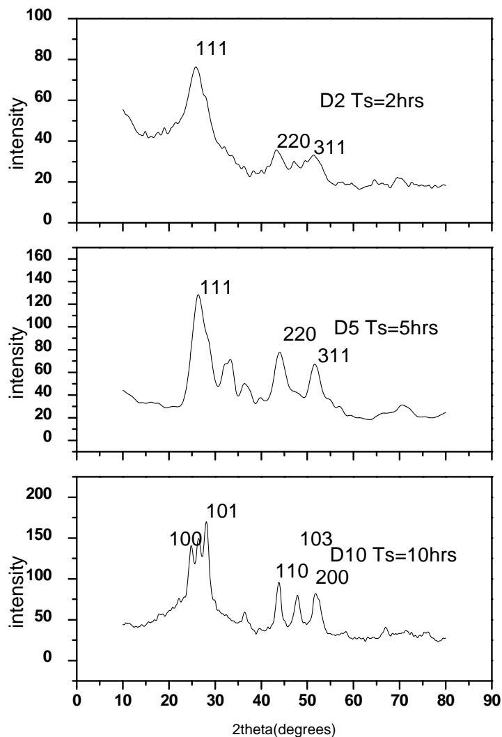
Fig. 1 XRD profiles of CdS nanocrystals
