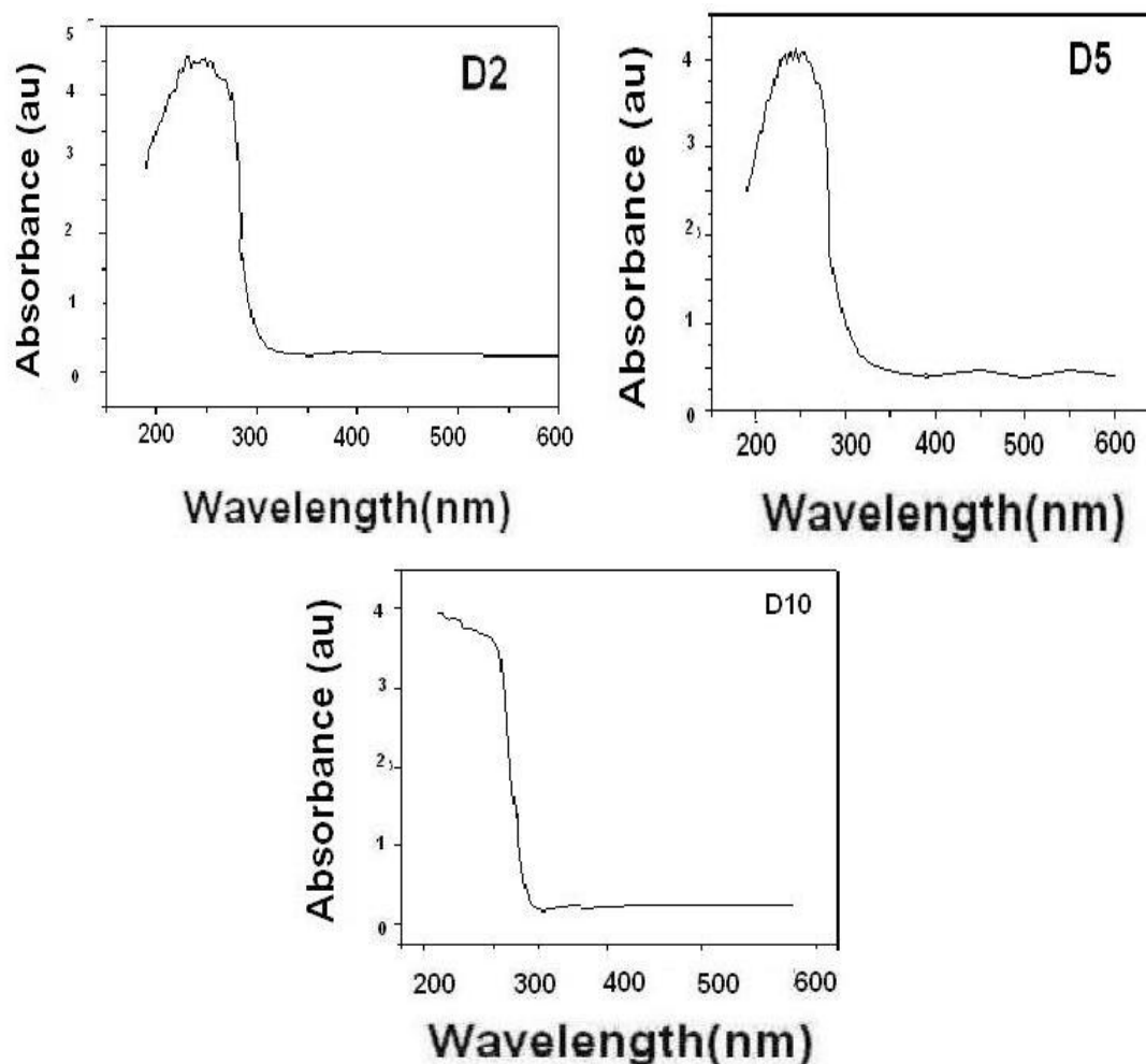
Fig 3 Absorbance spectra of CdS nanocrystals
